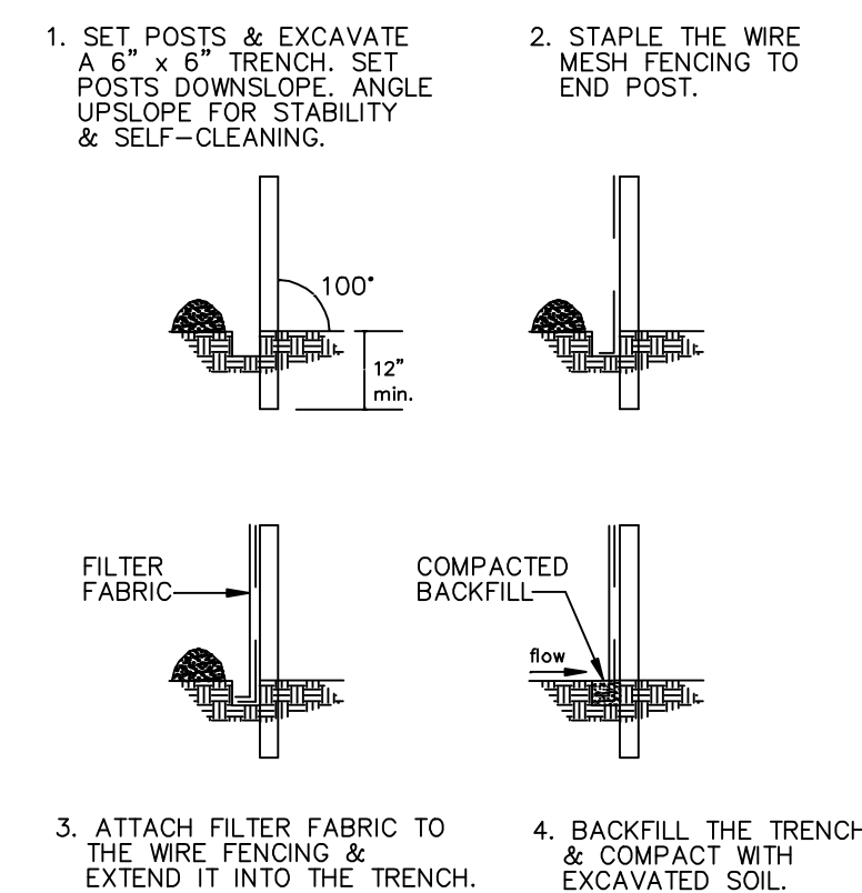
FILTER FABRIC SEDIMENT BARRIER NOT TO SCALE
