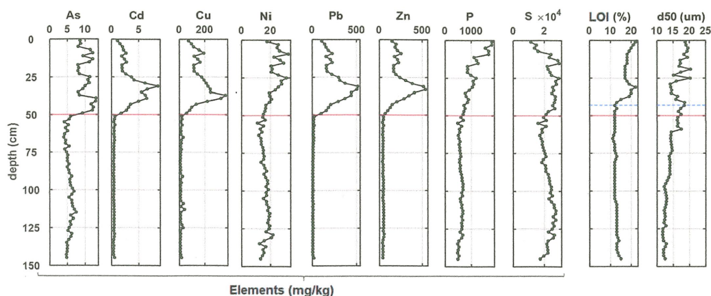
Fig. 9. Down-core profiles from our estuary sediment core showing concentrations of metals (As, Cd, Cu, Ni, Pb, Zn), phosphorous, sulfur, percent organic (LOI), and median grain size (d50). The depth at which metals increase above background is indicated by a red line, and corresponds to the onset of industrialization in the region.
