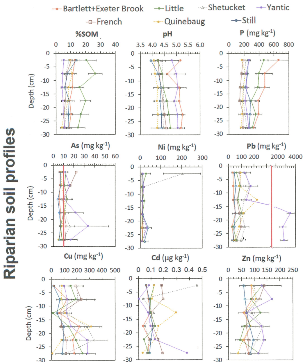
Fig. 2. Riparian soil trace metal concentrations collected from 27 stream banks across the seven subwatersheds. Error bars represent standard error among the riparian soils sampled in each watershed. Red lines for As and Pb indicate CT-DEEP limits for direct exposure for humans; limits for Ni, Cu, Cd, and Zn are not visible at the provided scale.
