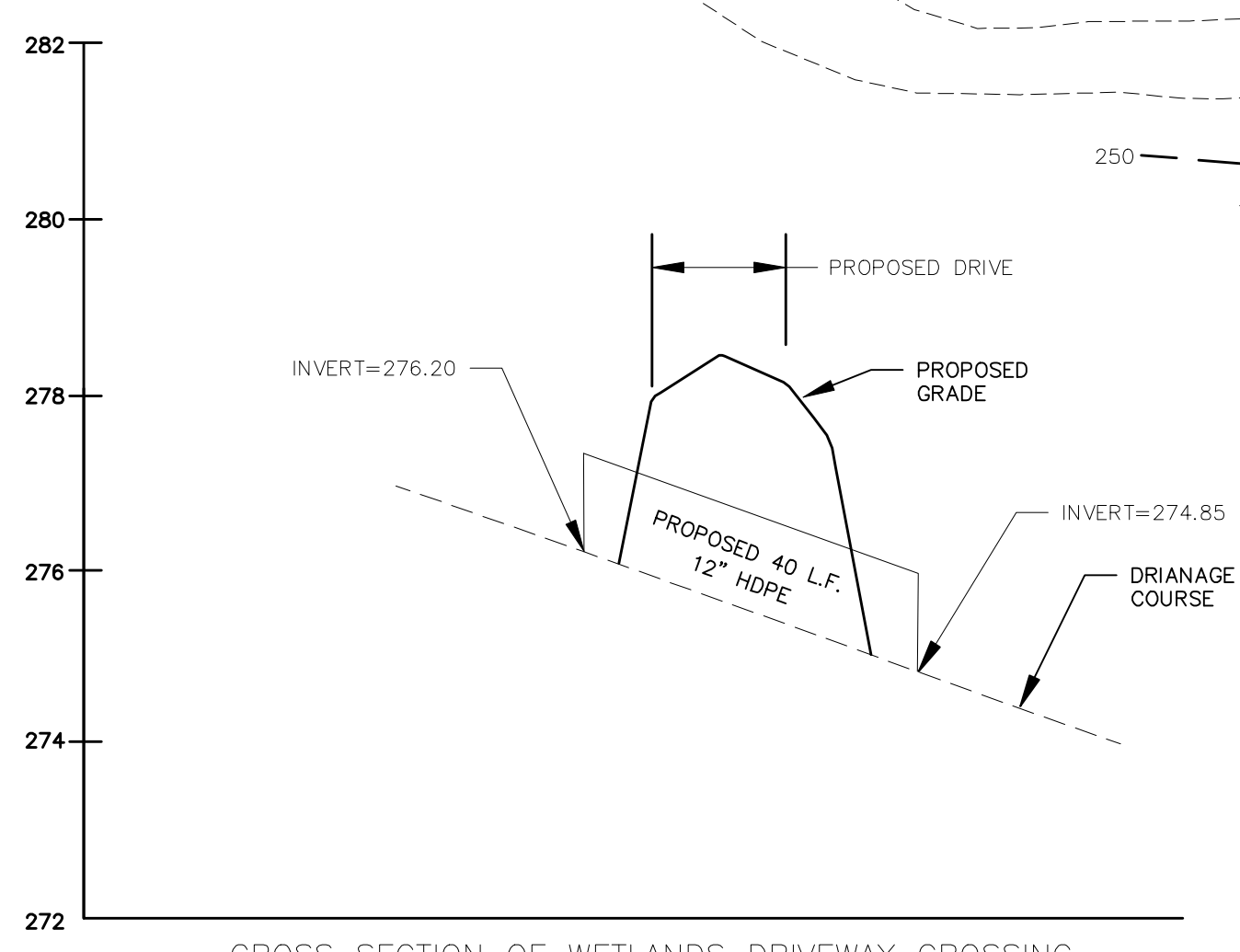
CROSS SECTION OF WETLANDS DRIVEWAY CROSSING SCALE: 1"=20'
