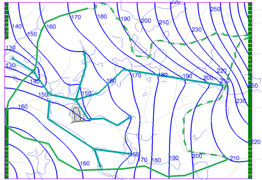
COMPUTED GROUNDWATER CONTOURS (PRESENT CONDITION)
