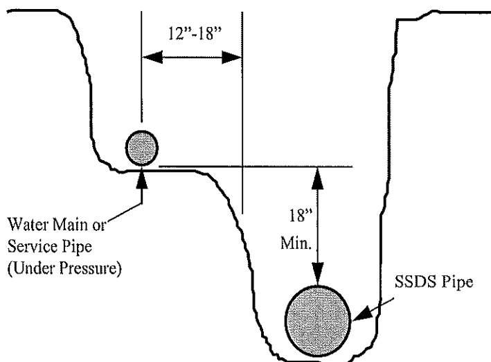
Figure 2 - Pressurized Water Pipe and SSDS Pipe Trenches
