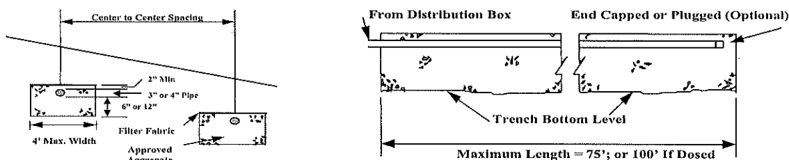
Figure 14 - Leaching Trenches
