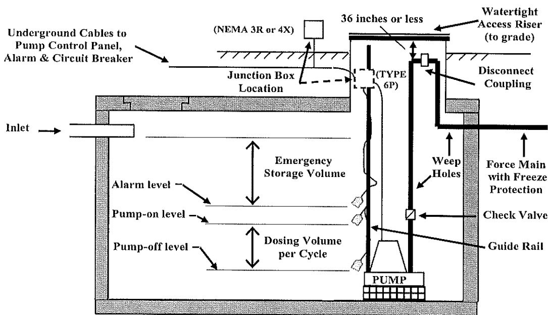
Figure 11 - Pump Chamber
