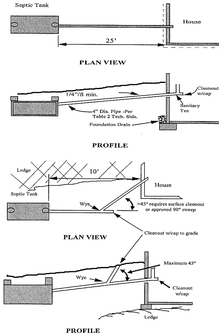
Figure 1 - Building Sewers
