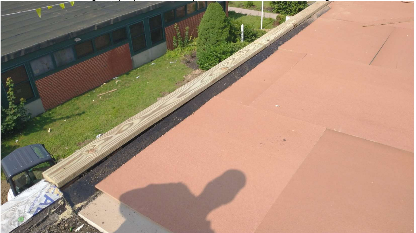
Roof B – PT board for raising of the parapet since the roof pitch was not discovered until the roofing material was removed
