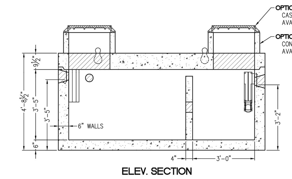
1,250 GALLON HS-20 SEPTIC TANK NOT TO SCALE
