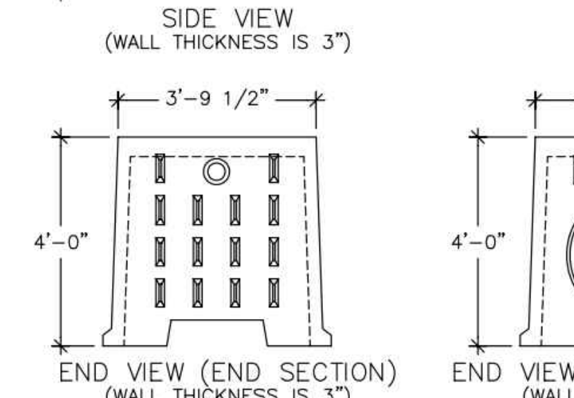
48" HIGH HS-20 LEACHING GALLEY NOT TO SCALE
